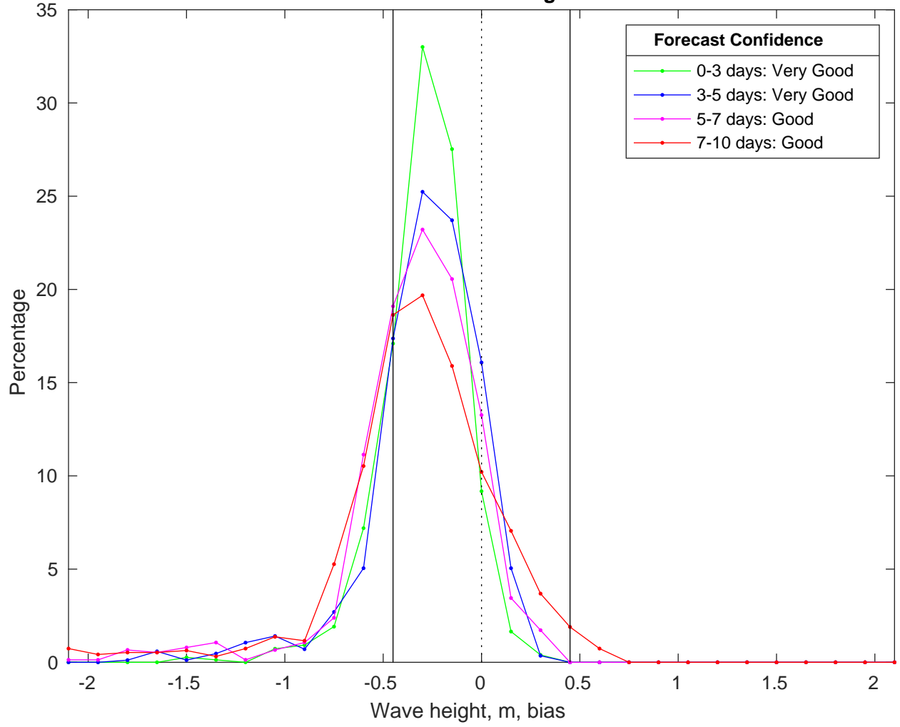
NDBC 52213 vs CMEMS Waves Bias Histogram: 14-Mar-2025
