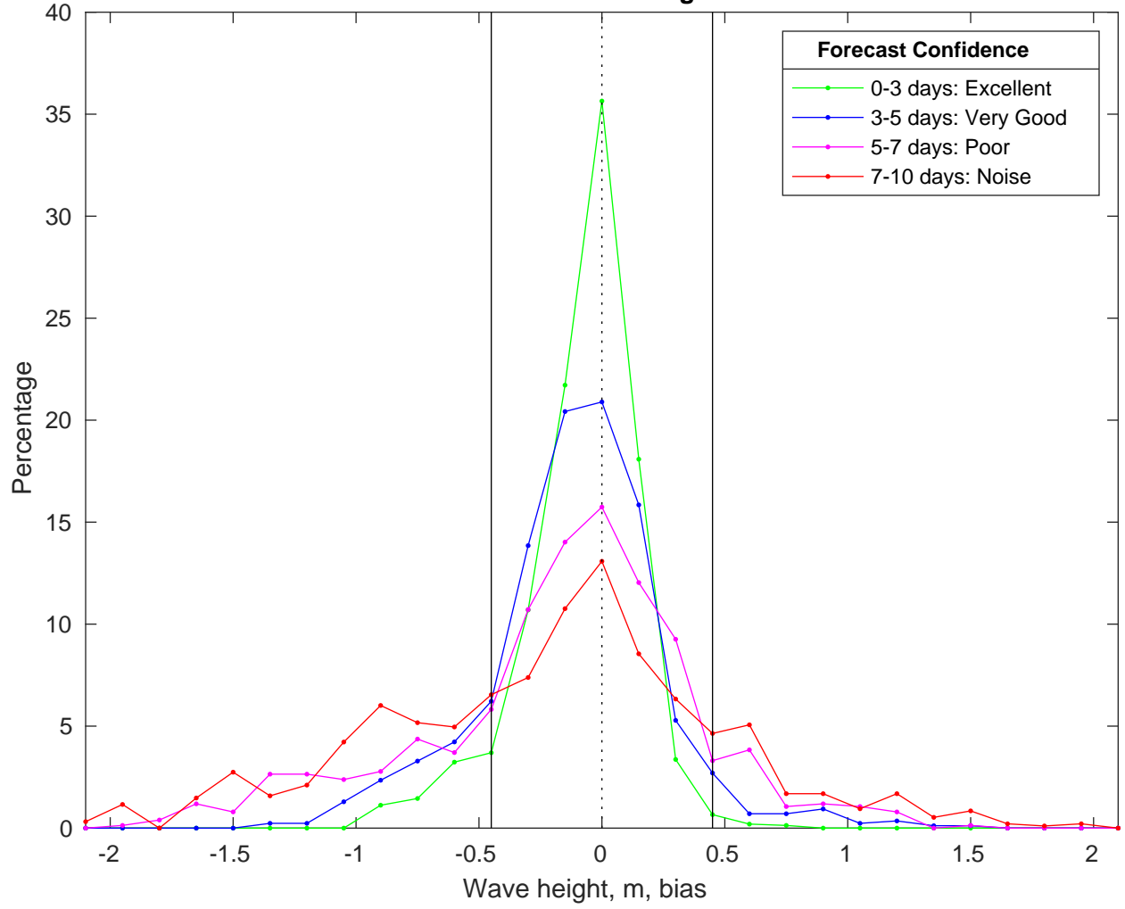
NDBC 41004 vs CMEMS Waves Bias Histogram: 15-Mar-2025
