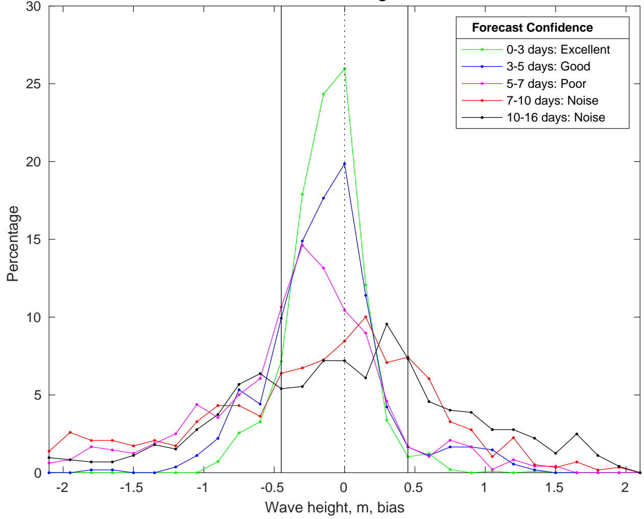
NDBC 41004 vs GFS Waves Bias Histogram: 15-Mar-2025
