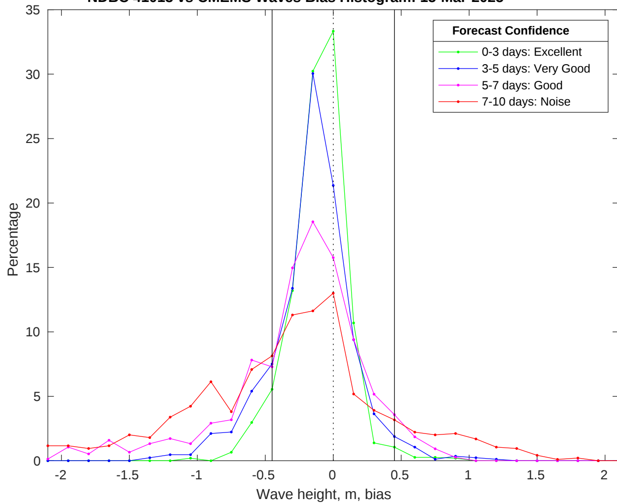
NDBC 41013 vs CMEMS Waves Bias Histogram: 15-Mar-2025
