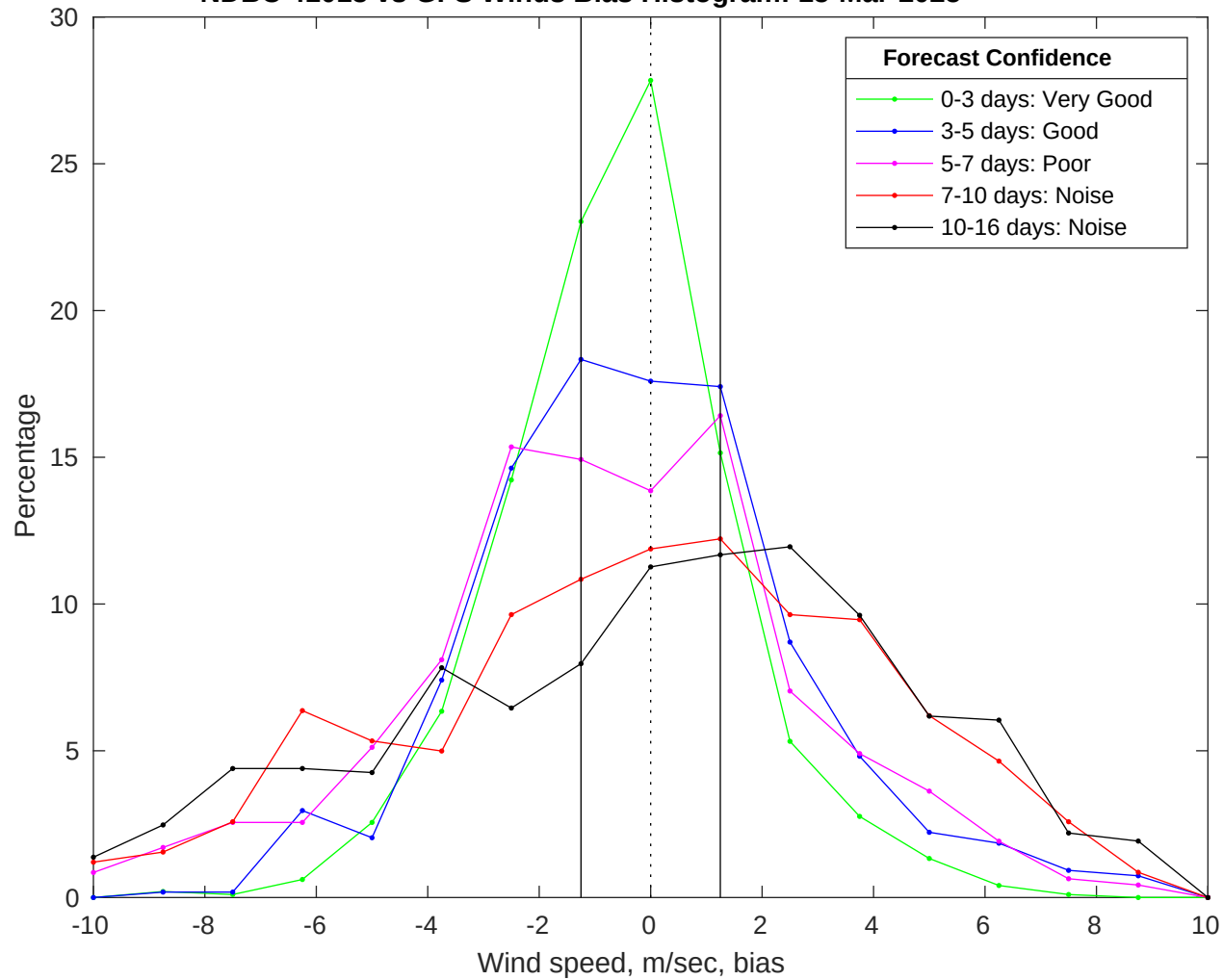
NDBC 41013 vs GFS Winds Bias Histogram: 15-Mar-2025
