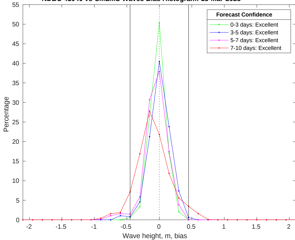
NDBC 41040 vs CMEMS Waves Bias Histogram: 15-Mar-2025
