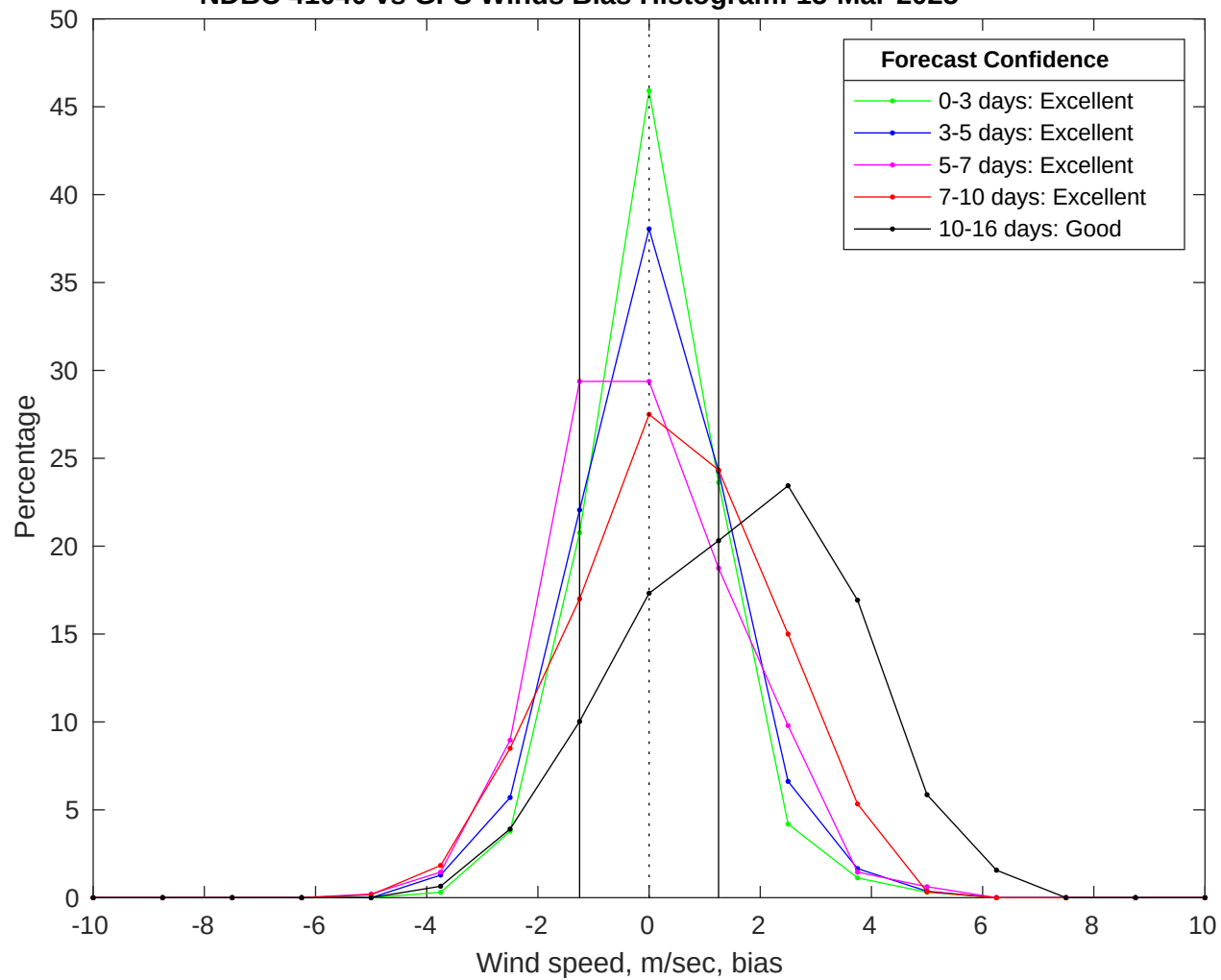
NDBC 41040 vs GFS Winds Bias Histogram: 15-Mar-2025
