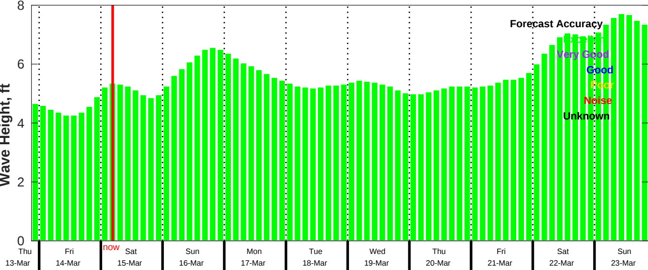
CMEMS Wave Forecast for NDBC 41040 from 13-Mar-2025 21:00:00 to 23-Mar-2025 21:00:00
