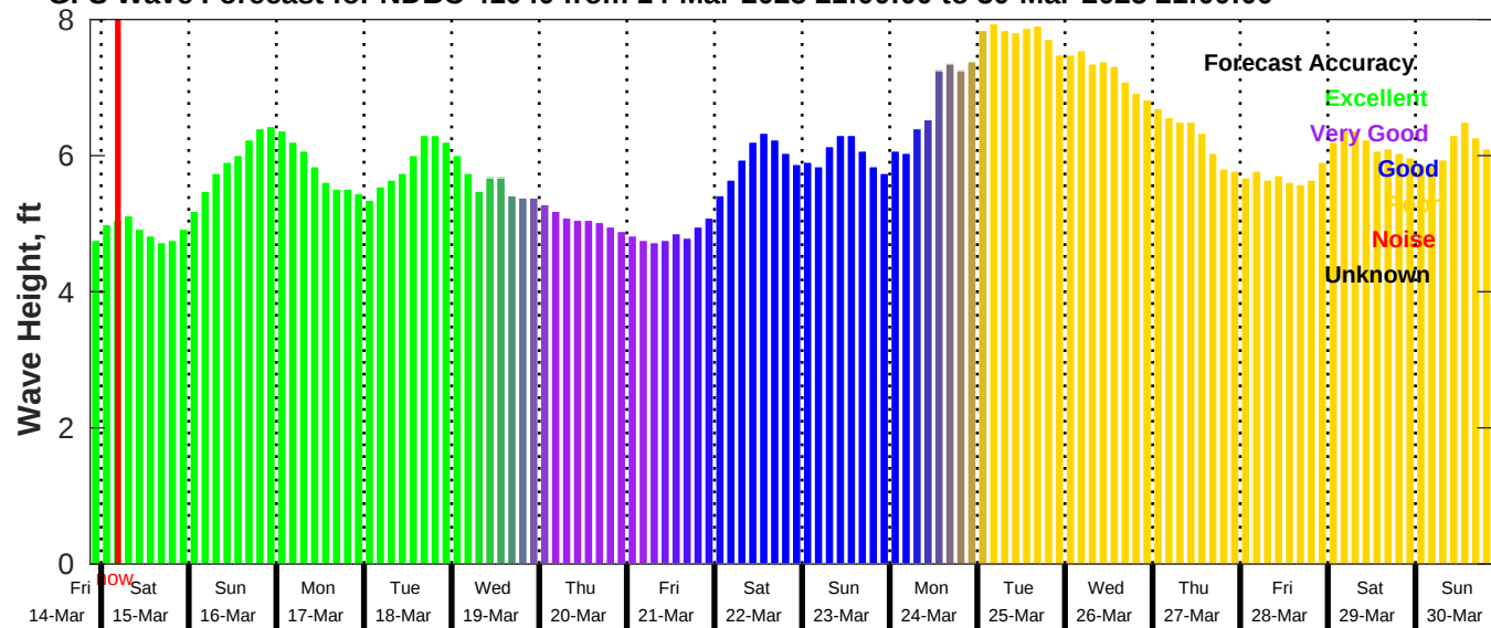
GFS Wave Forecast for NDBC 41040 from 14-Mar-2025 21:00:00 to 30-Mar-2025 21:00:00
