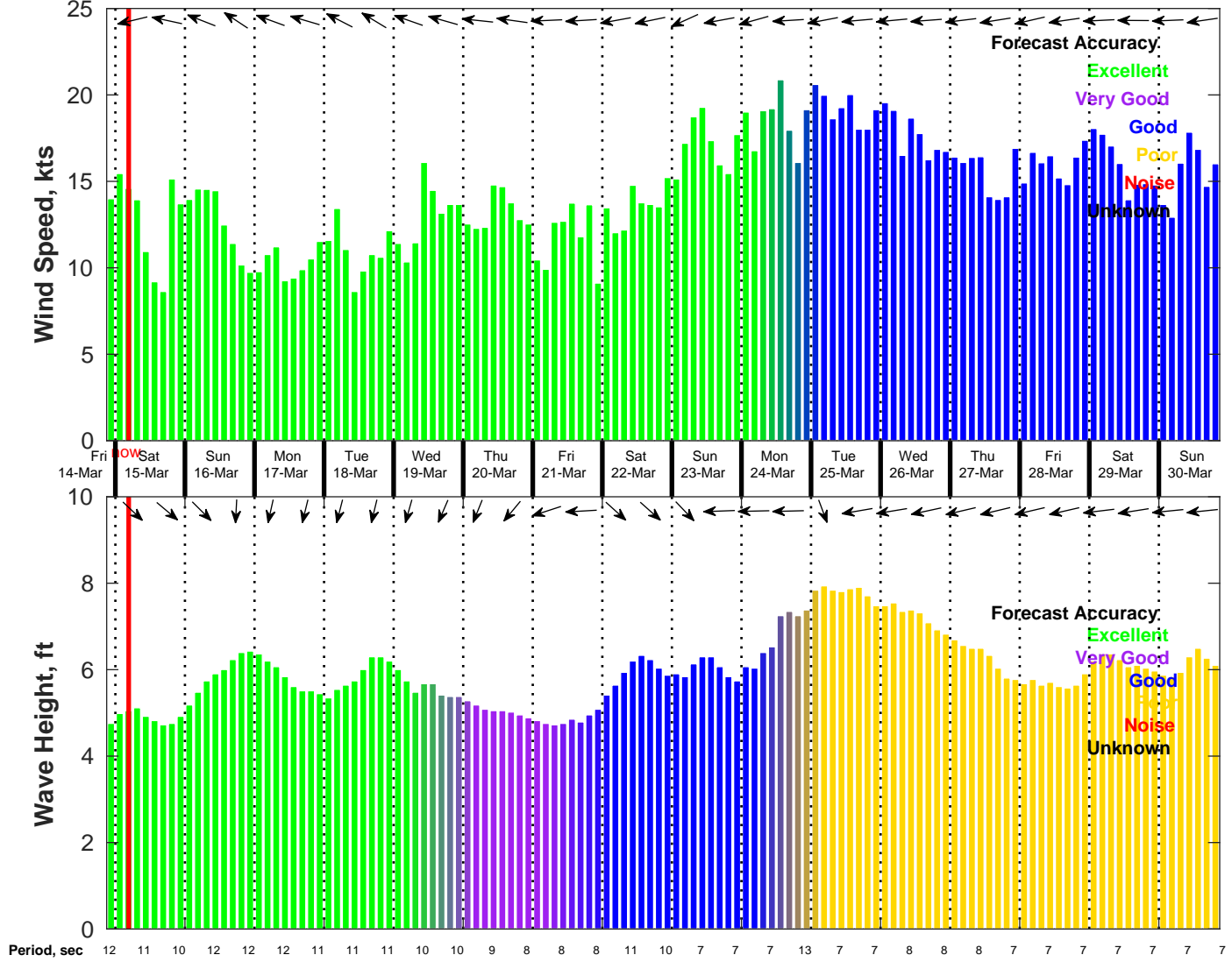
Wind & Wave Forecast for NDBC 41040 from 14-Mar-2025 21:00:00 to 30-Mar-2025 21:00:00
