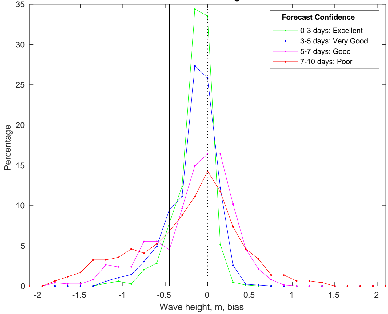
NDBC 42019 vs CMEMS Waves Bias Histogram: 15-Mar-2025
