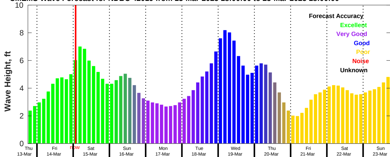
CMEMS Wave Forecast for NDBC 42019 from 13-Mar-2025 18:00:00 to 23-Mar-2025 18:00:00
