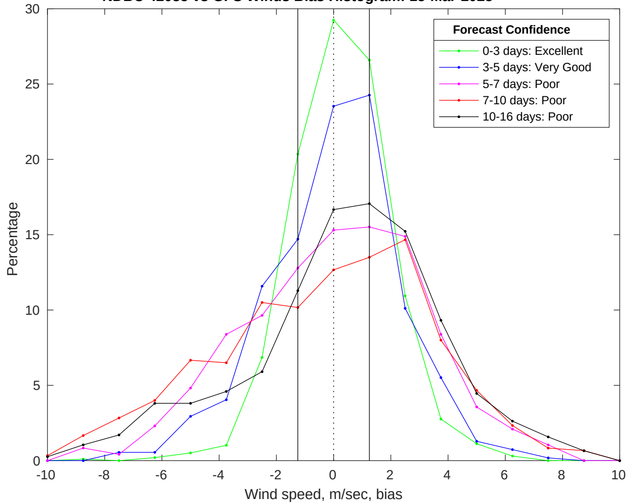
NDBC 42035 vs GFS Winds Bias Histogram: 15-Mar-2025
