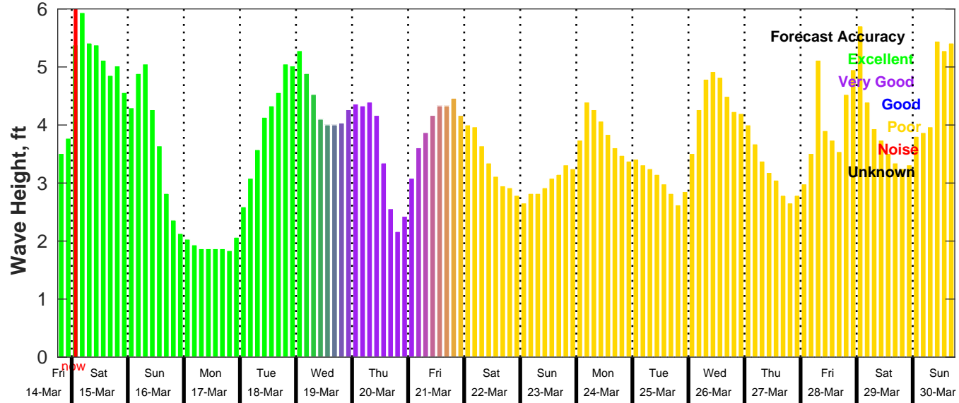
GFS Wave Forecast for NDBC 42035 from 14-Mar-2025 18:00:00 to 30-Mar-2025 18:00:00
