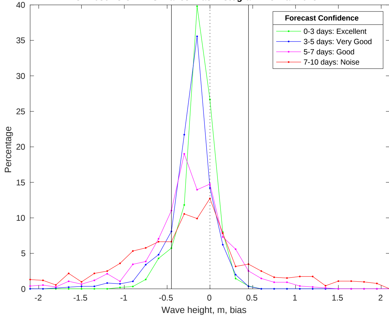
NDBC 42036 vs CMEMS Waves Bias Histogram: 15-Mar-2025
