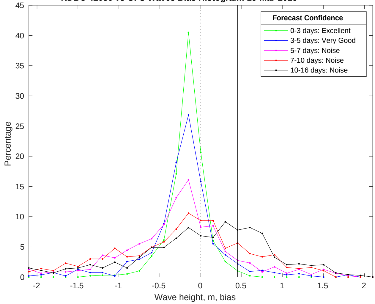
NDBC 42036 vs GFS Waves Bias Histogram: 15-Mar-2025
