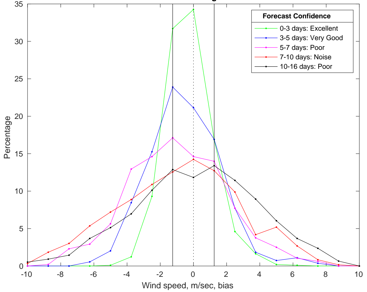
NDBC 42036 vs GFS Winds Bias Histogram: 15-Mar-2025
