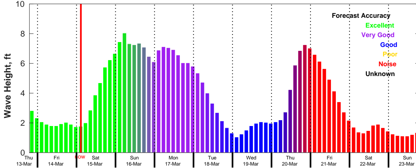
CMEMS Wave Forecast for NDBC 42036 from 13-Mar-2025 19:00:00 to 23-Mar-2025 19:00:00
