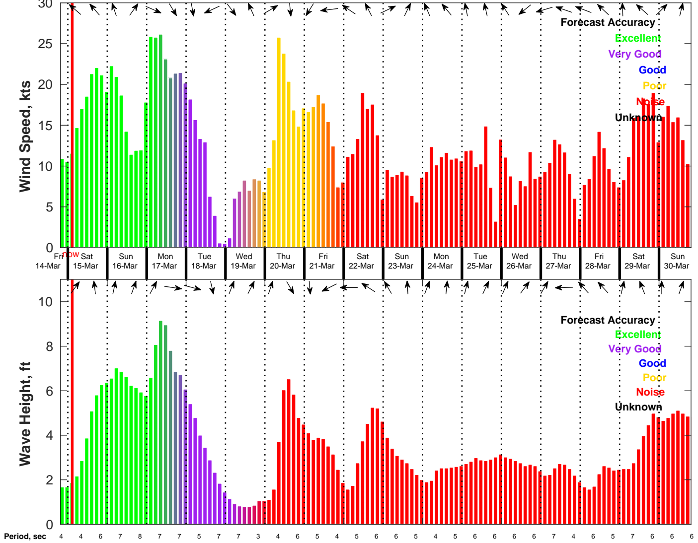
Wind & Wave Forecast for NDBC 42036 from 14-Mar-2025 19:00:00 to 30-Mar-2025 19:00:00
