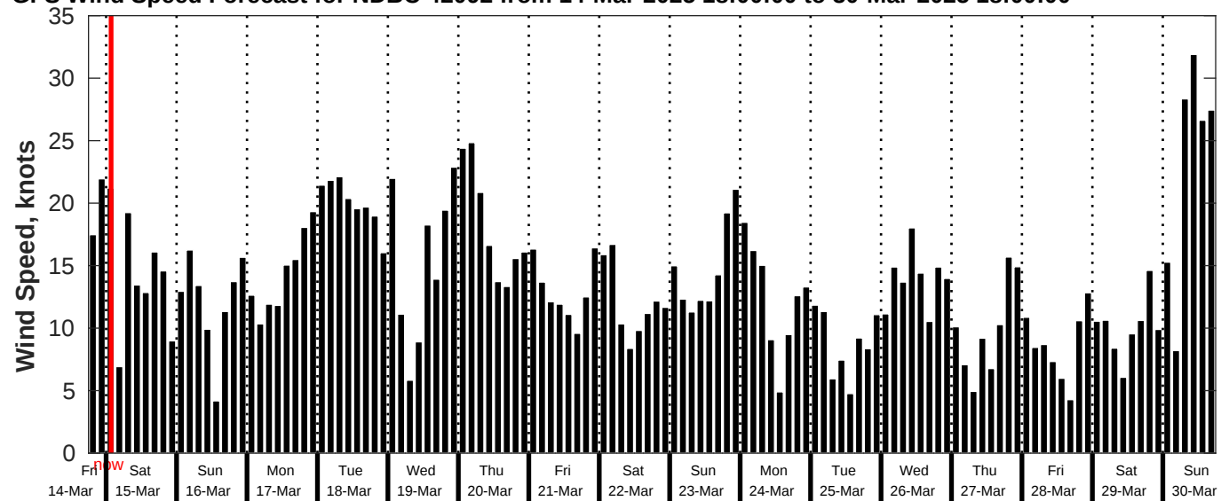
GFS Wind Speed Forecast for NDBC 42092 from 14-Mar-2025 18:00:00 to 30-Mar-2025 18:00:00
