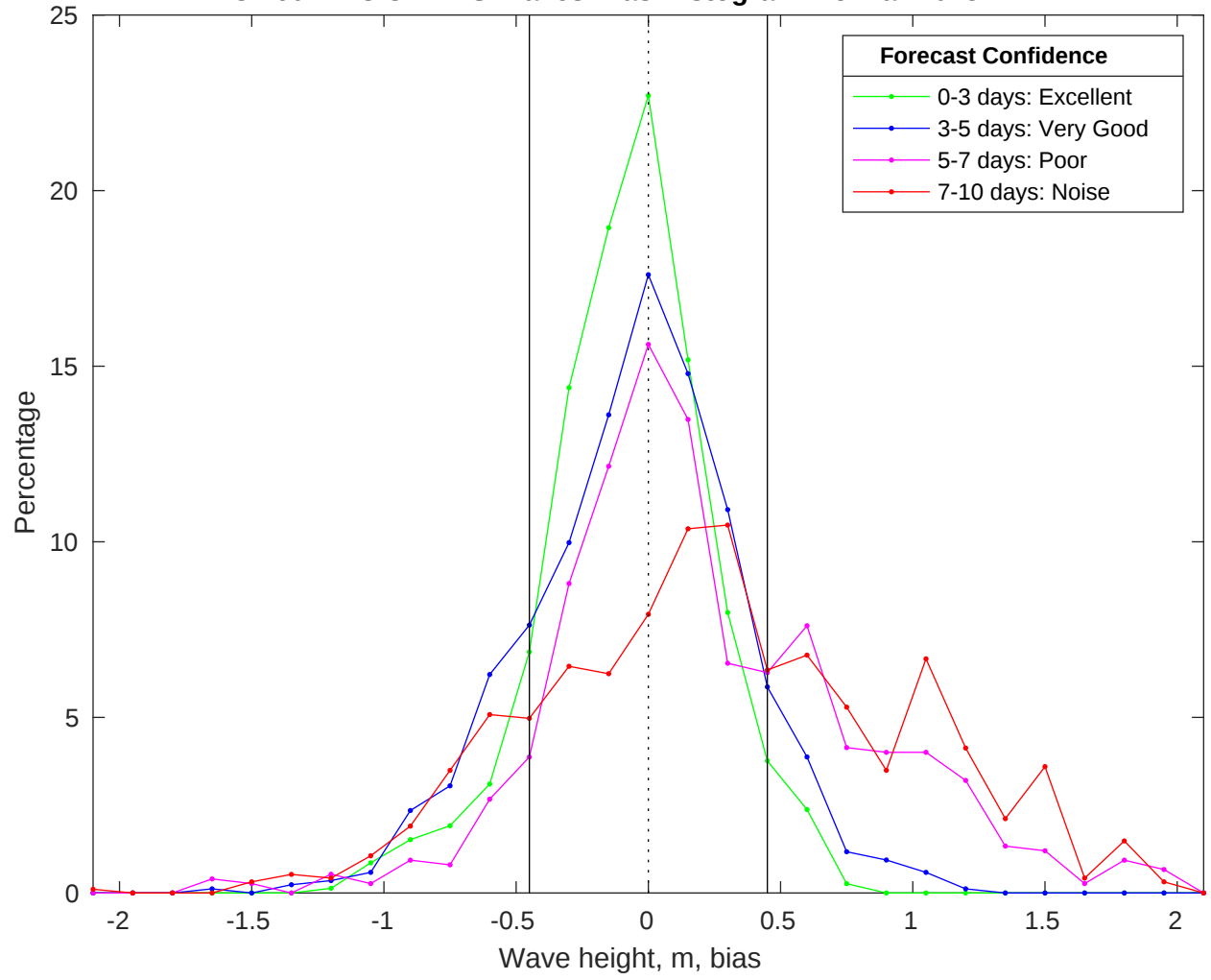
NDBC 46011 vs CMEMS Waves Bias Histogram: 15-Mar-2025
