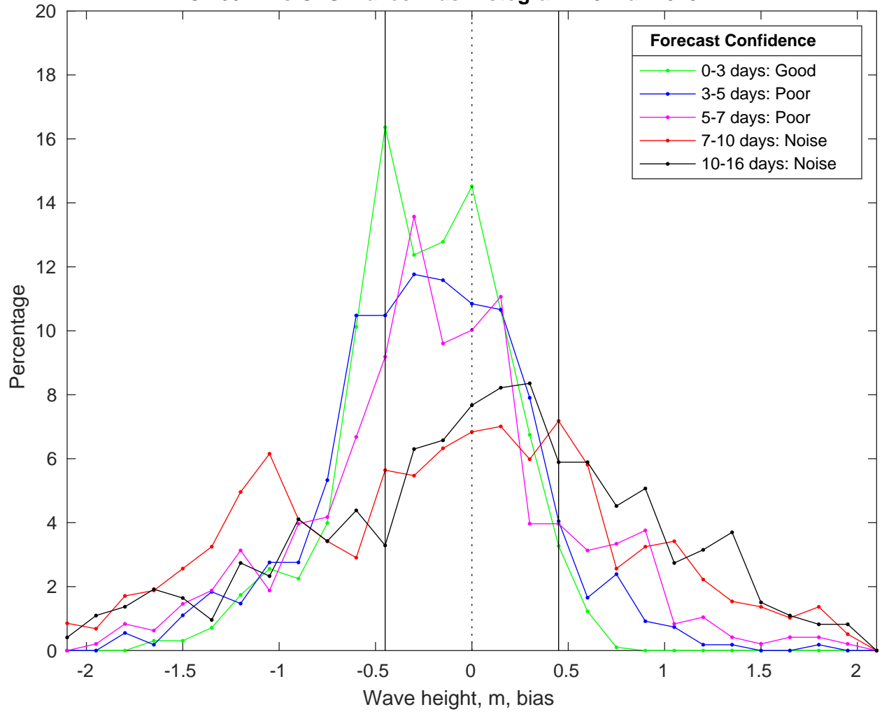
NDBC 46011 vs GFS Waves Bias Histogram: 15-Mar-2025
