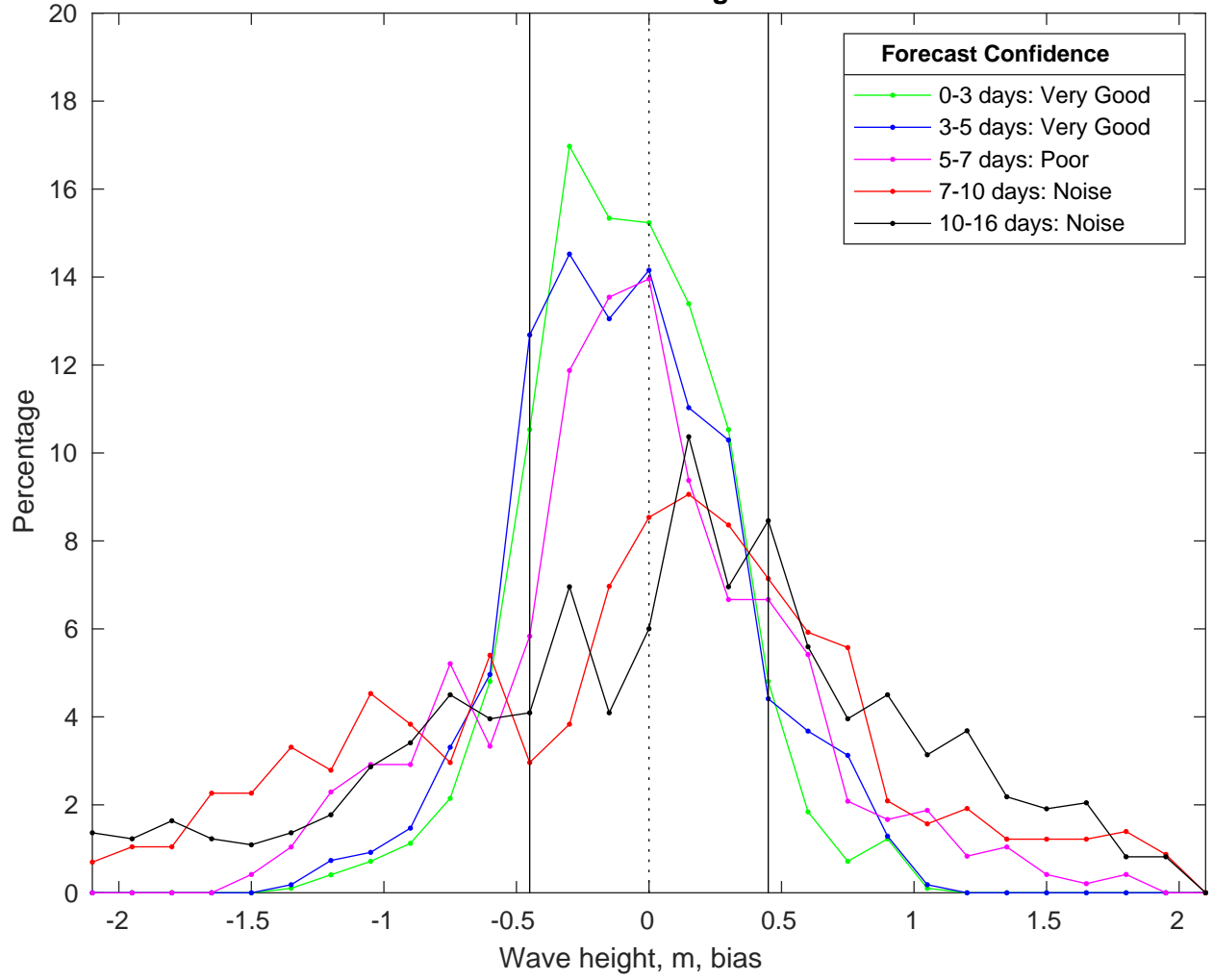
NDBC 46028 vs GFS Waves Bias Histogram: 15-Mar-2025
