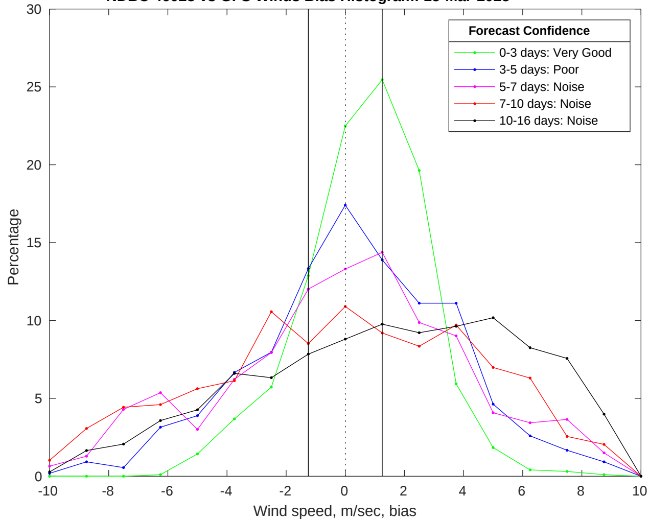
NDBC 46028 vs GFS Winds Bias Histogram: 15-Mar-2025
