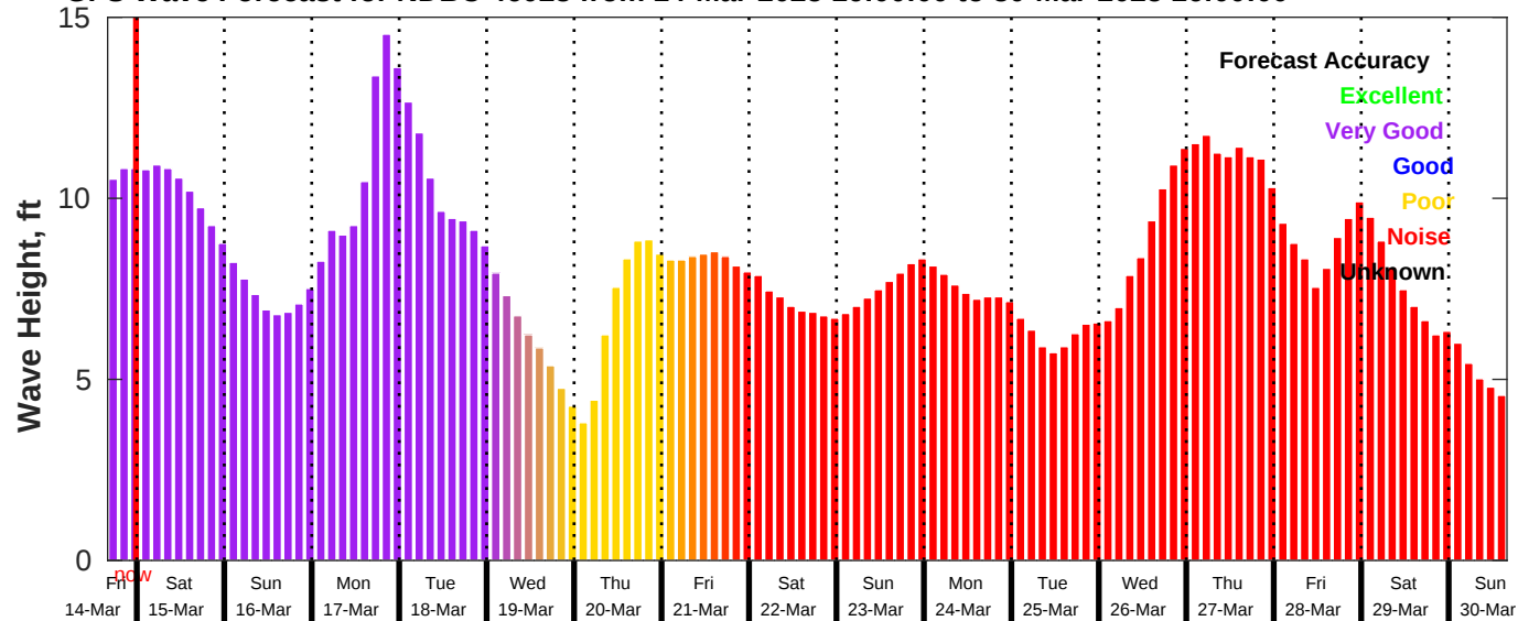
GFS Wave Forecast for NDBC 46028 from 14-Mar-2025 16:00:00 to 30-Mar-2025 16:00:00
