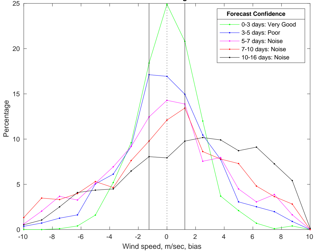
NDBC 46054 vs GFS Winds Bias Histogram: 15-Mar-2025
