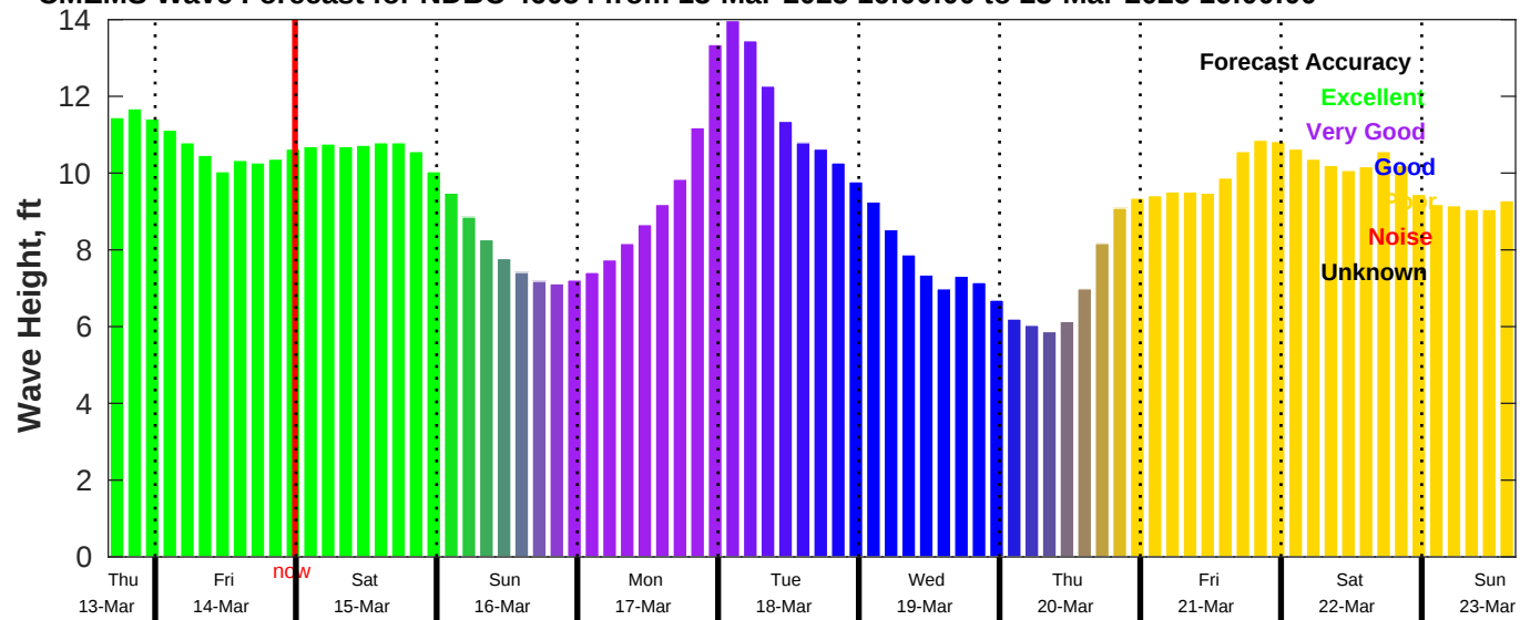
CMEMS Wave Forecast for NDBC 46054 from 13-Mar-2025 16:00:00 to 23-Mar-2025 16:00:00
