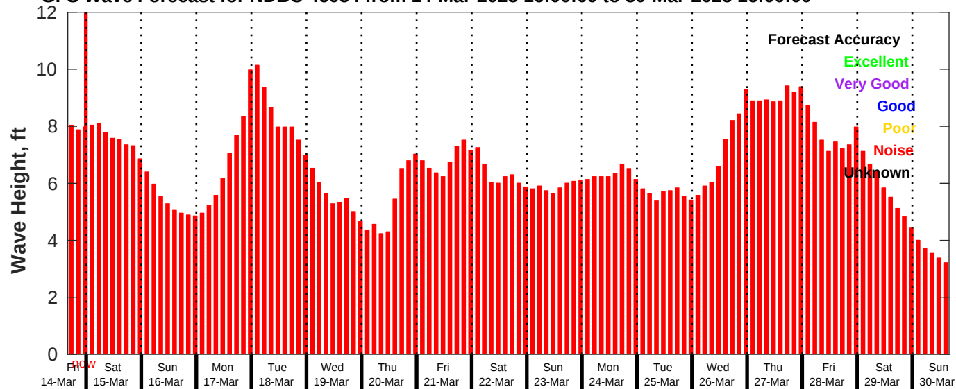
GFS Wave Forecast for NDBC 46054 from 14-Mar-2025 16:00:00 to 30-Mar-2025 16:00:00
