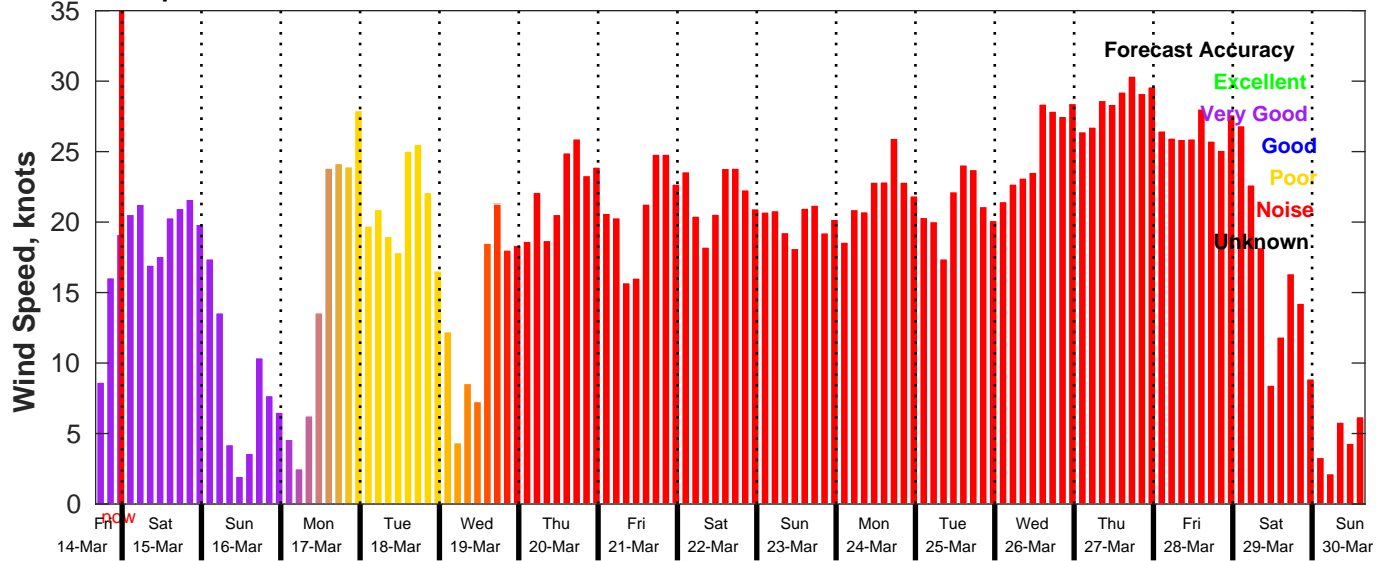
GFS Wind Speed Forecast for NDBC 46054 from 14-Mar-2025 16:00:00 to 30-Mar-2025 16:00:00
