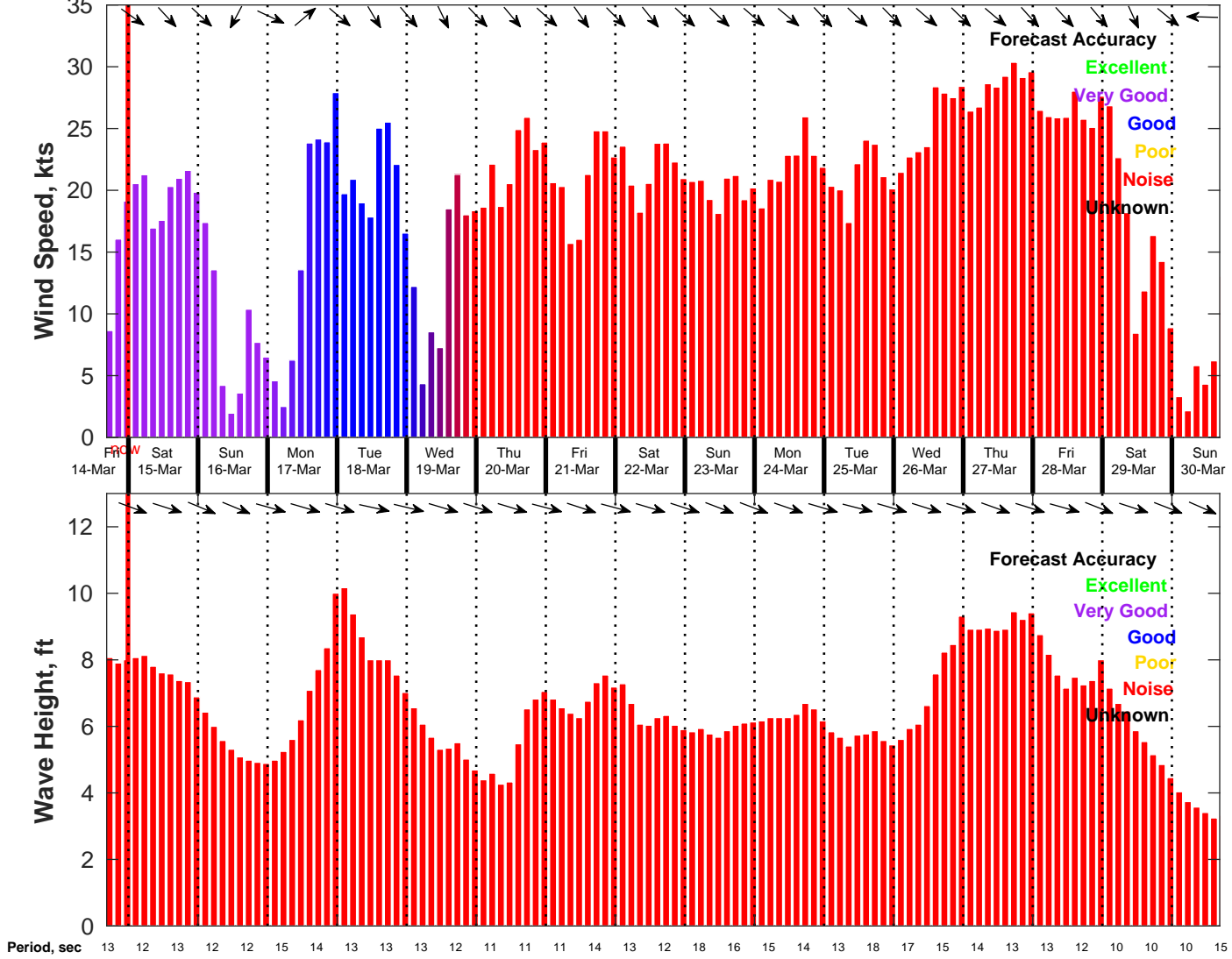
Wind & Wave Forecast for NDBC 46054 from 14-Mar-2025 16:00:00 to 30-Mar-2025 16:00:00
