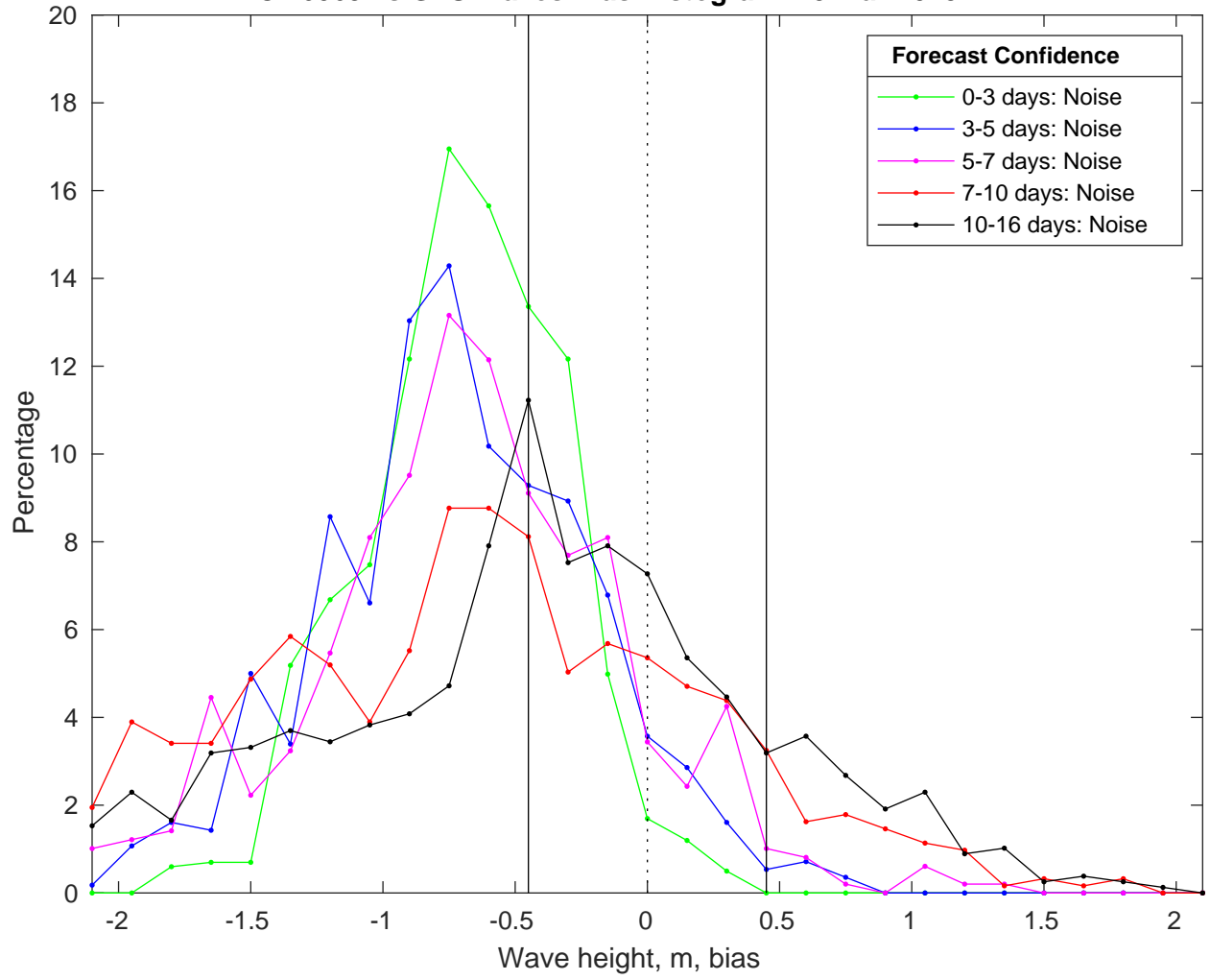
NDBC 46069 vs GFS Waves Bias Histogram: 15-Mar-2025
