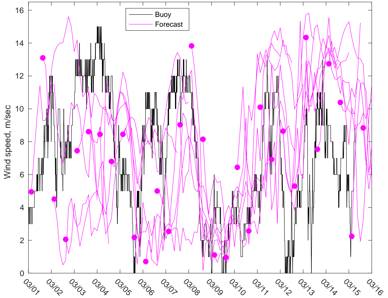
NDBC 46069 vs GFS Winds: 7 to 10 day forecast
