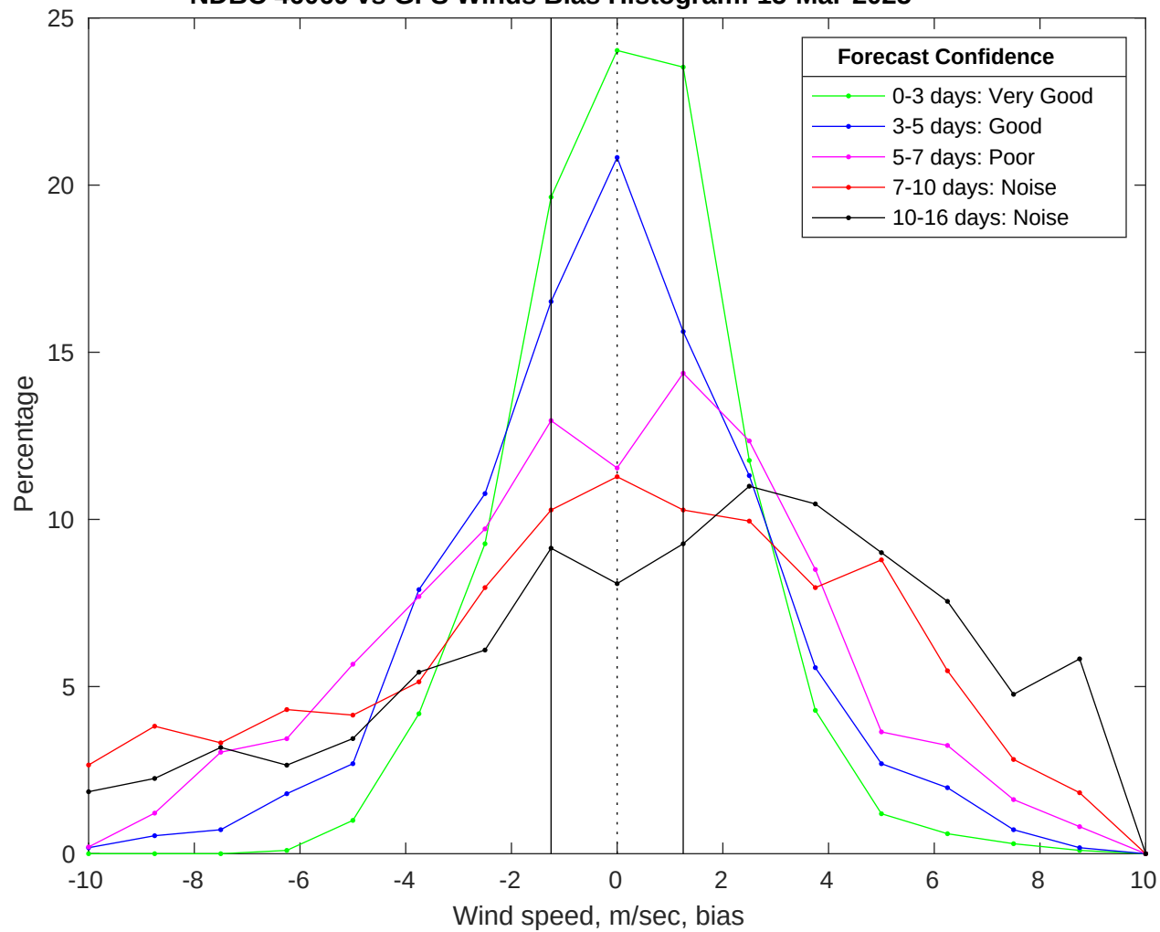
NDBC 46069 vs GFS Winds Bias Histogram: 15-Mar-2025
