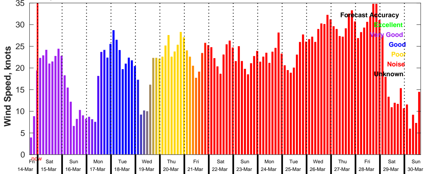
GFS Wind Speed Forecast for NDBC 46069 from 14-Mar-2025 16:00:00 to 30-Mar-2025 16:00:00
