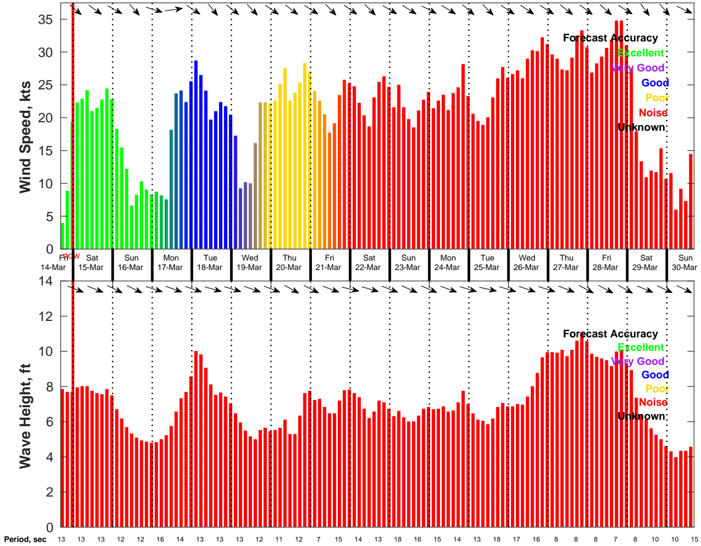
Wind & Wave Forecast for NDBC 46069 from 14-Mar-2025 16:00:00 to 30-Mar-2025 16:00:00
