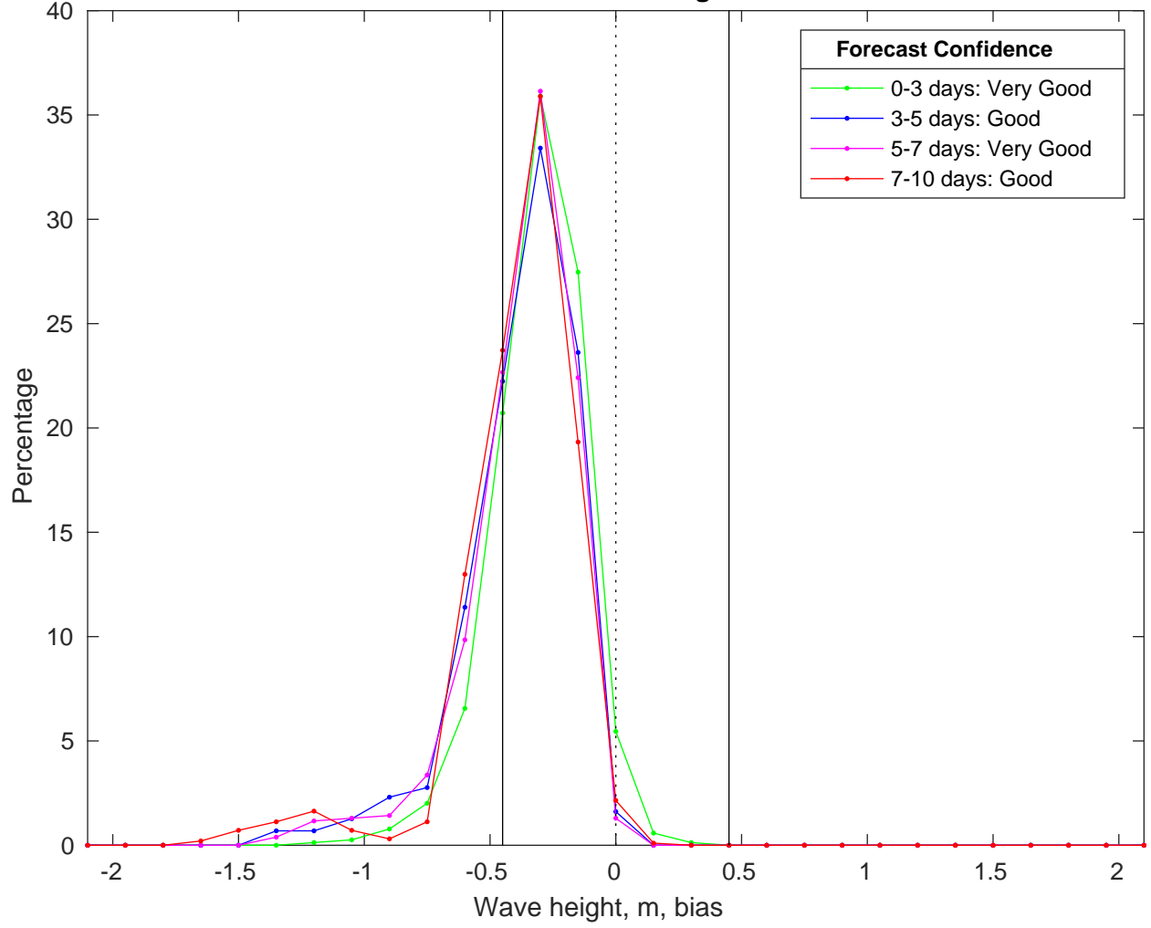
NDBC 51209 vs CMEMS Waves Bias Histogram: 15-Mar-2025
