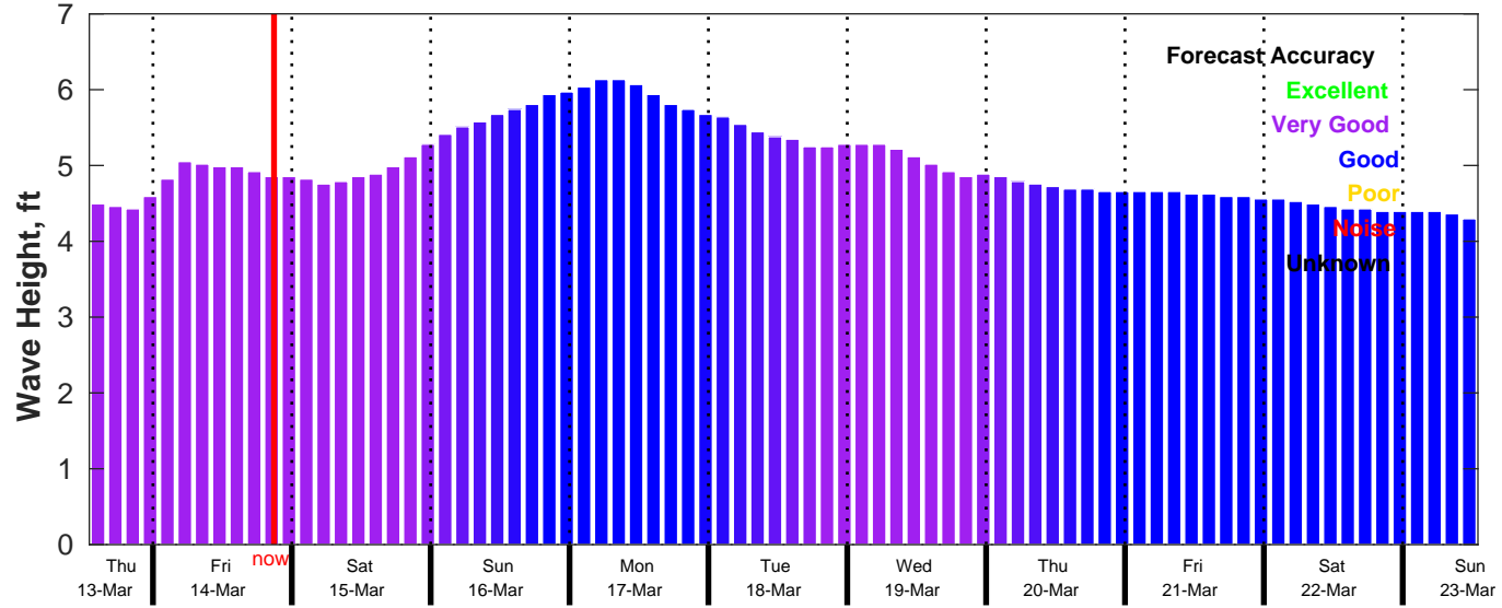
CMEMS Wave Forecast for NDBC 51209 from 13-Mar-2025 13:00:00 to 23-Mar-2025 13:00:00
