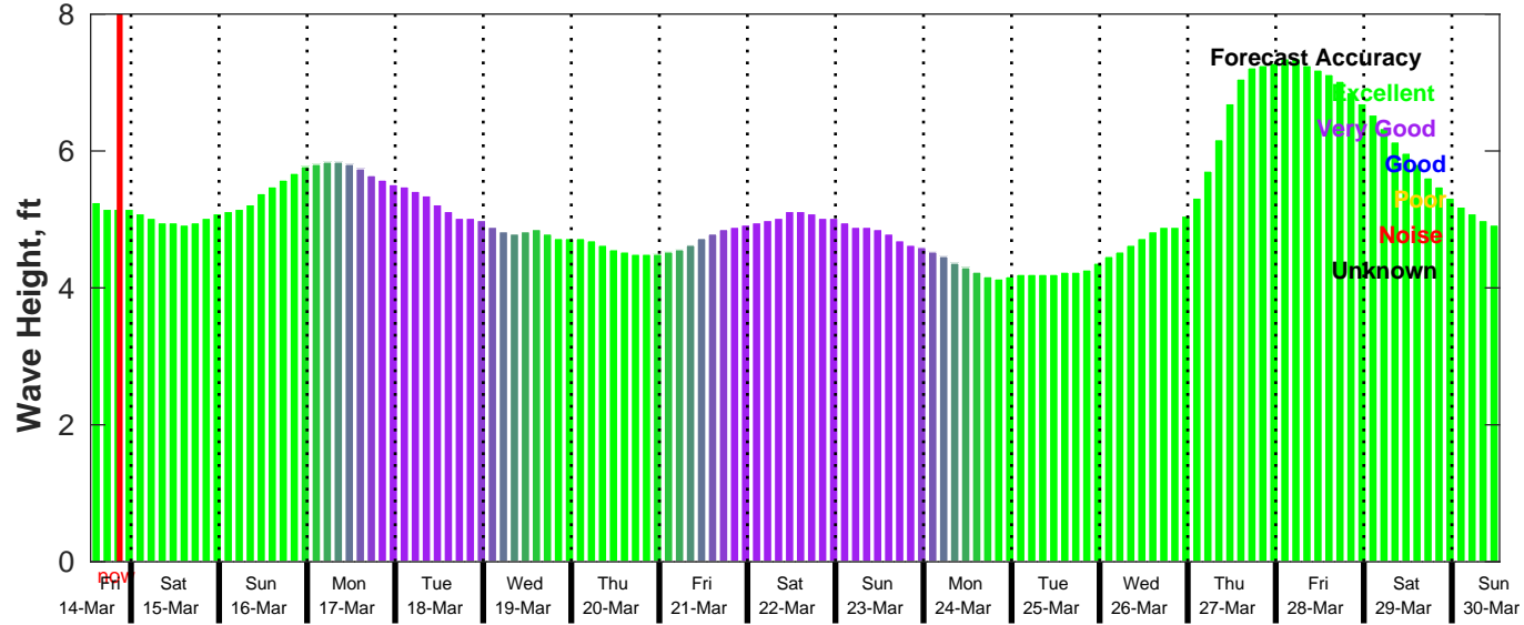
GFS Wave Forecast for NDBC 51209 from 14-Mar-2025 13:00:00 to 30-Mar-2025 13:00:00
