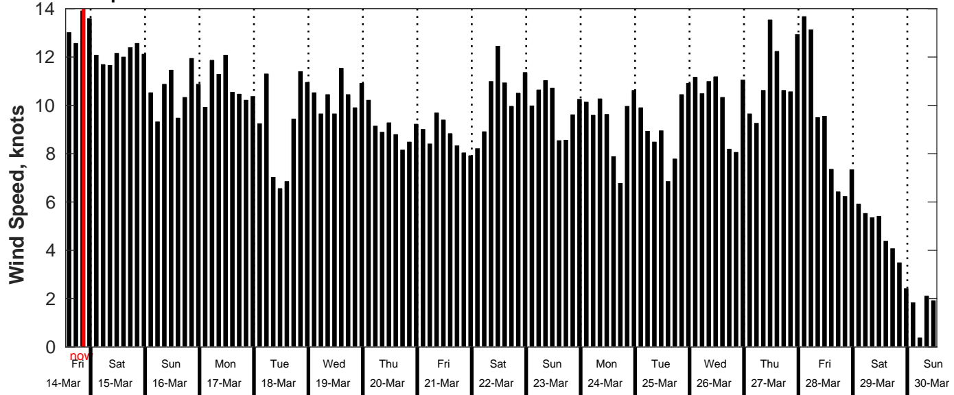
GFS Wind Speed Forecast for NDBC 51209 from 14-Mar-2025 13:00:00 to 30-Mar-2025 13:00:00
