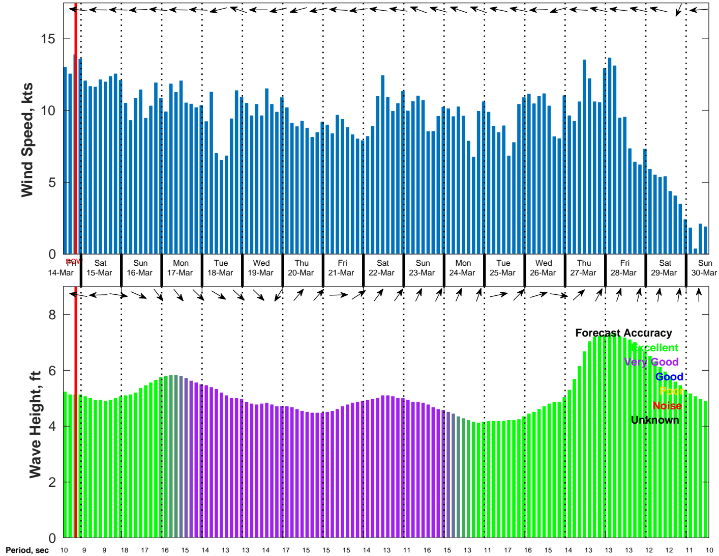
Wind & Wave Forecast for NDBC 51209 from 14-Mar-2025 13:00:00 to 30-Mar-2025 13:00:00
