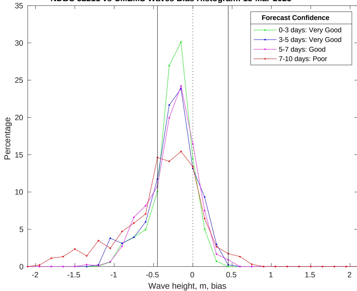
NDBC 52211 vs CMEMS Waves Bias Histogram: 15-Mar-2025
