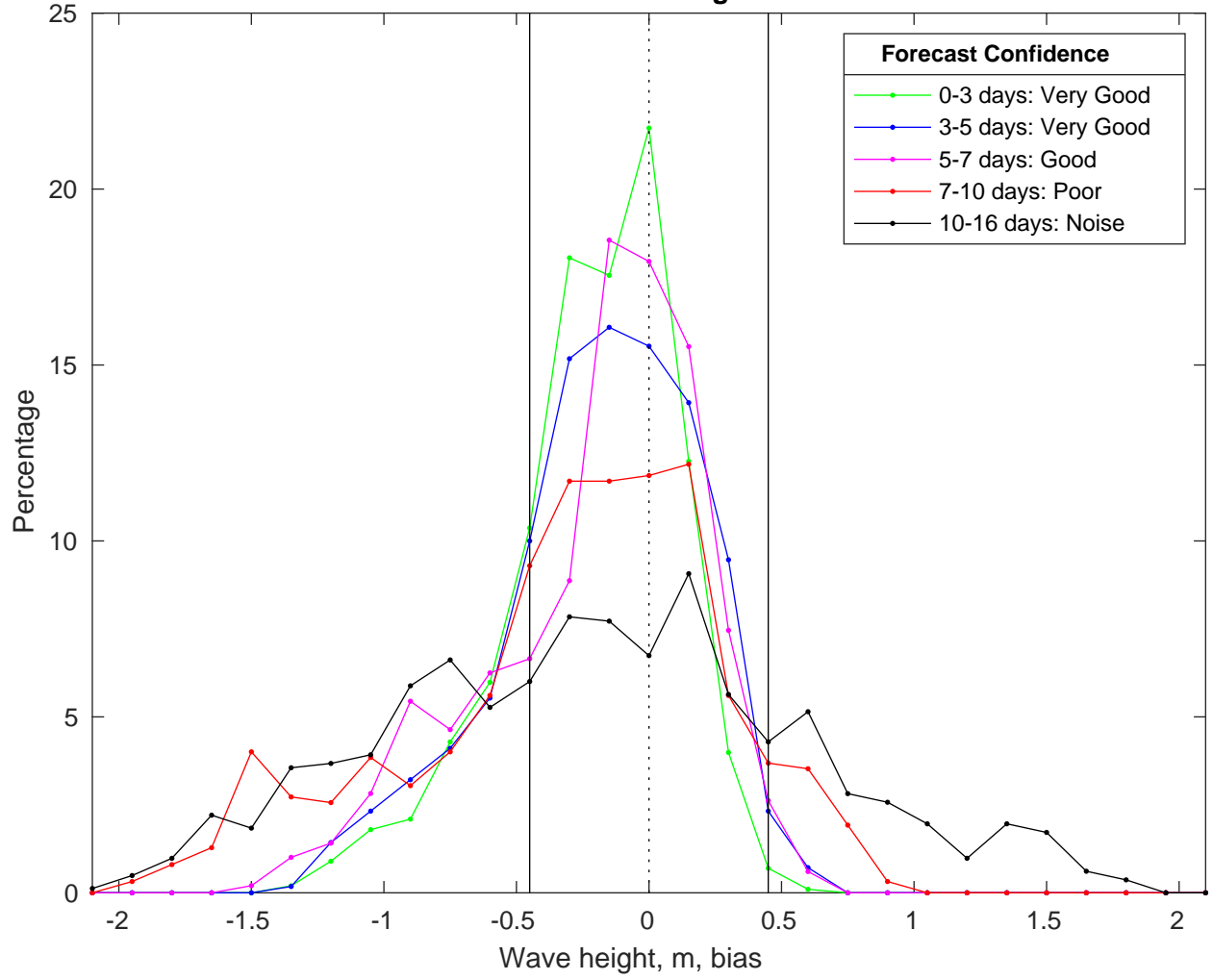
NDBC 52211 vs GFS Waves Bias Histogram: 15-Mar-2025
