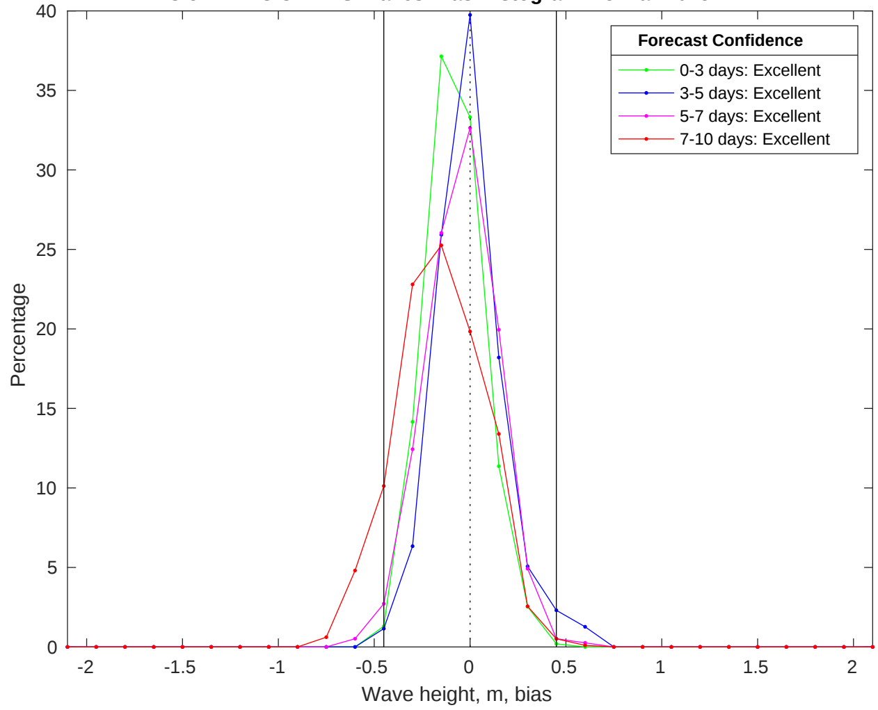
NDBC 52212 vs CMEMS Waves Bias Histogram: 15-Mar-2025
