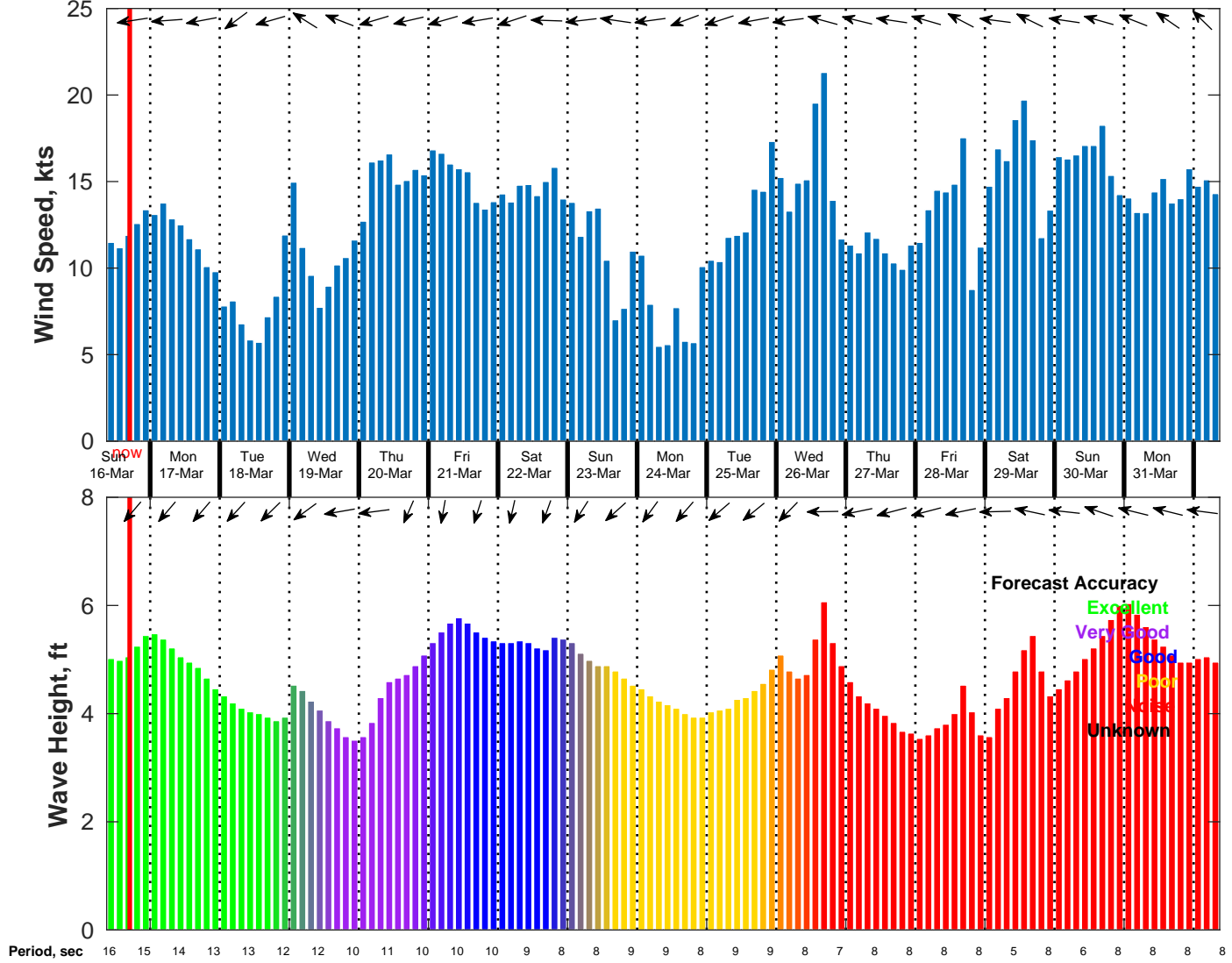
Wind & Wave Forecast for NDBC 52212 from 15-Mar-2025 09:00:00 to 31-Mar-2025 09:00:00
