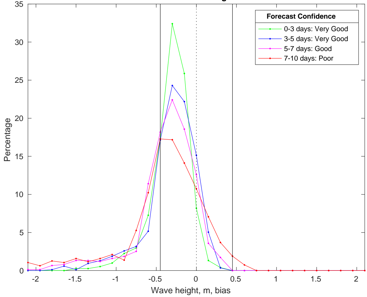
NDBC 52213 vs CMEMS Waves Bias Histogram: 15-Mar-2025
