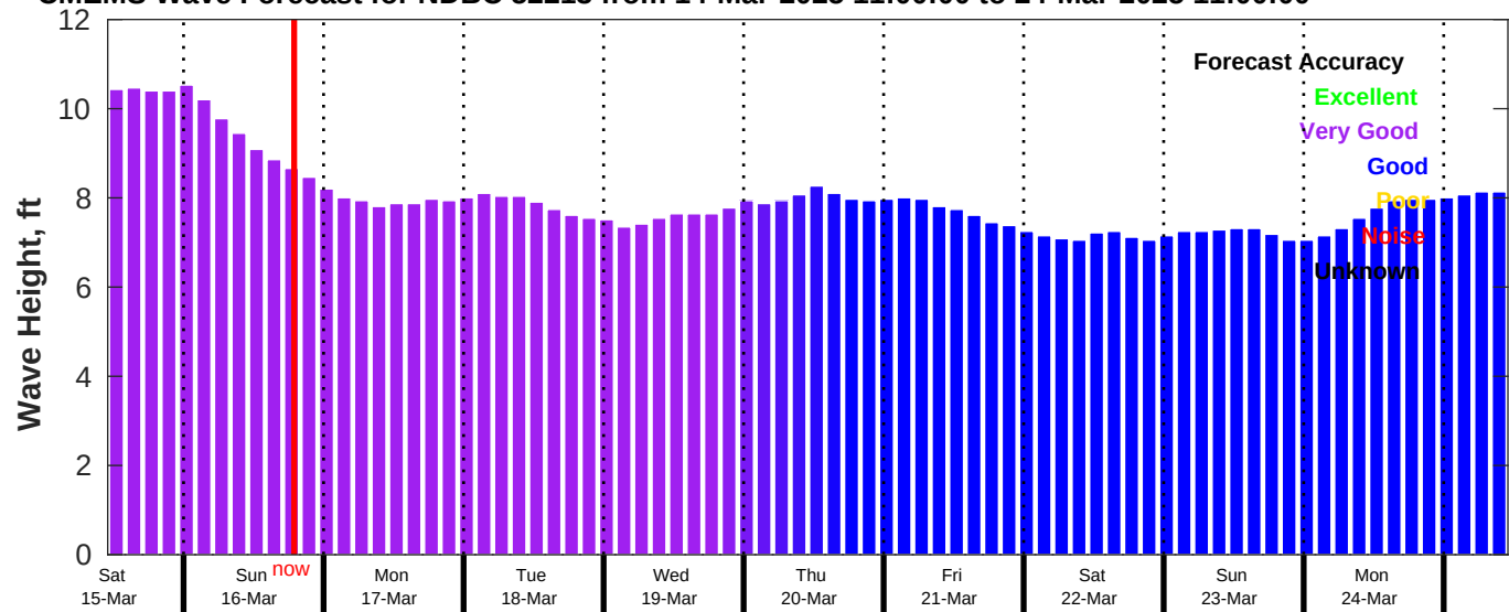
CMEMS Wave Forecast for NDBC 52213 from 14-Mar-2025 11:00:00 to 24-Mar-2025 11:00:00
