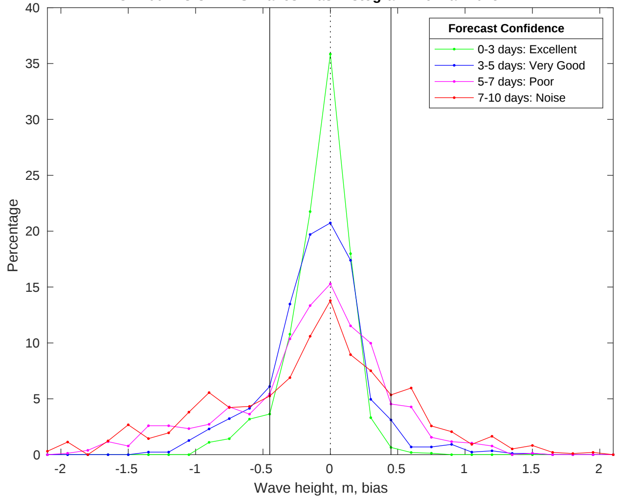
NDBC 41004 vs CMEMS Waves Bias Histogram: 16-Mar-2025
