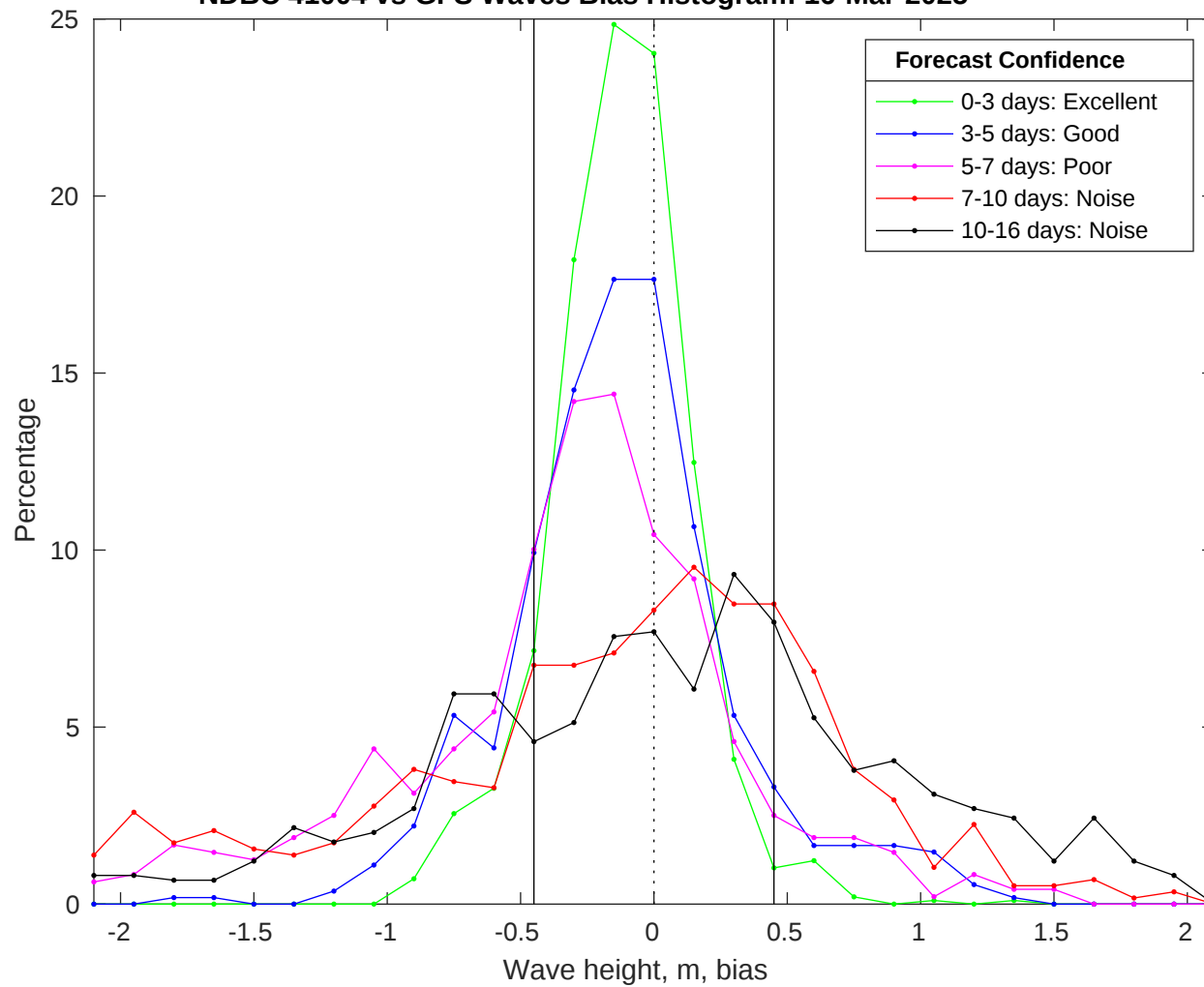
NDBC 41004 vs GFS Waves Bias Histogram: 16-Mar-2025
