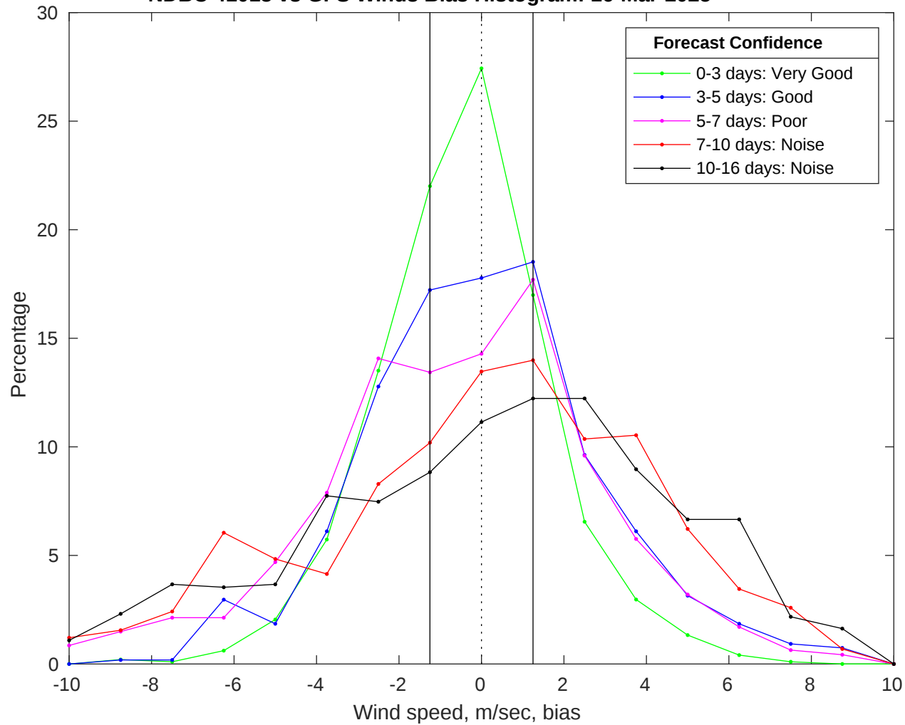
NDBC 41013 vs GFS Winds Bias Histogram: 16-Mar-2025
