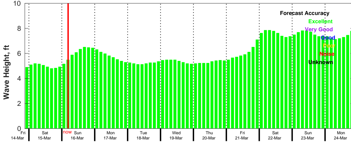
CMEMS Wave Forecast for NDBC 41040 from 14-Mar-2025 21:00:00 to 24-Mar-2025 21:00:00
